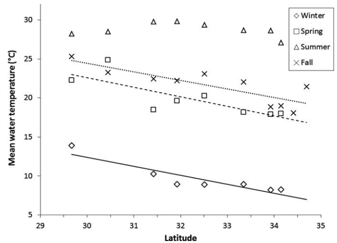
Fig. 4. The effect of latitude on mean water temperature by season. Temperature varied significantly with latitude during winter ( - ) [winter temperature = -1.15 \times \text{latitude} + 47.0 ]; spring ( - - - ) [spring temperature = -1.23 \times \text{latitude} + 59.5 ]; and fall ( - \cdot - \cdot - ) [fall temperature = -1.1 \times \text{latitude} + 57.4 ]. During summer, temperatures did not vary with latitude (summer temperature = -0.15 \times \text{latitude} + 33.6 ).
